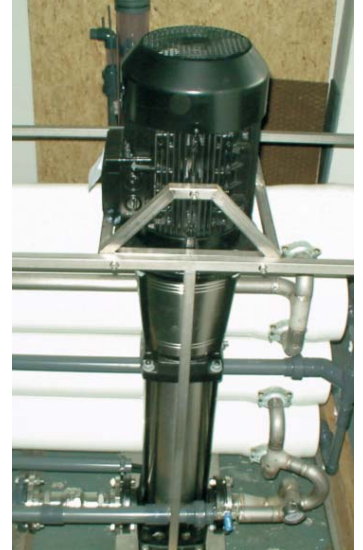
multistage high pressure pump
