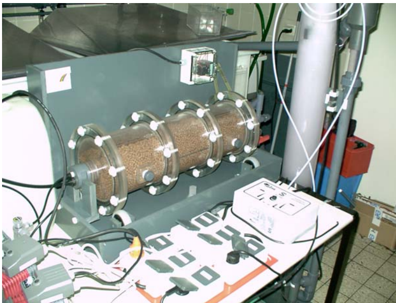
experimental unit with RBR 15, ACF 3000VC, dosing pumps and ozone generator connected to a 2 m 3 fish tank
