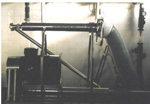
Multi stage high pressure pump with energy recovery turbine made of special steel 1.4462
