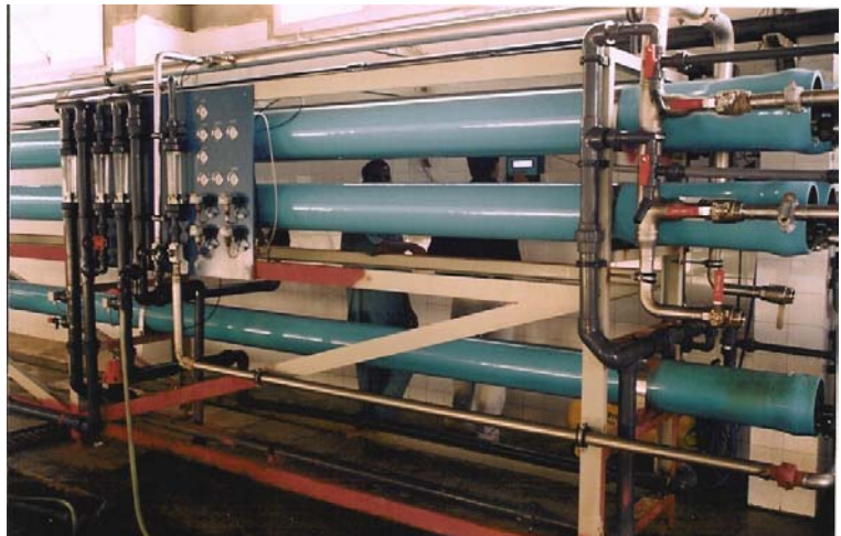
high pressure R.O. modules (65 bar)
